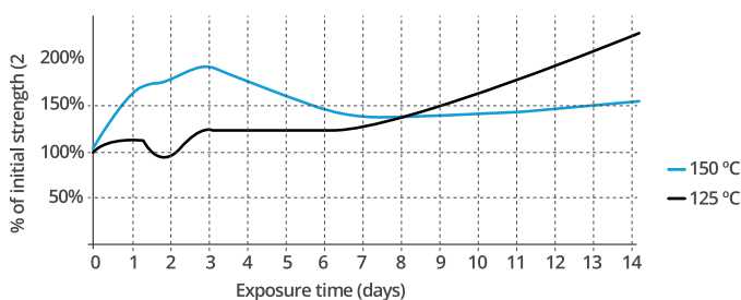
Adhesion Evolution On Mild Steel After Exposure To High Temperatures For Extended Periods
